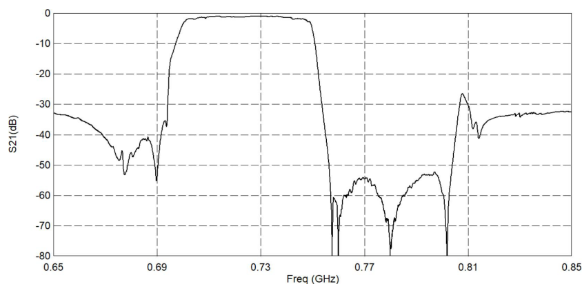
Figure 2 Electrical Characteristics: Tx to Ant.
