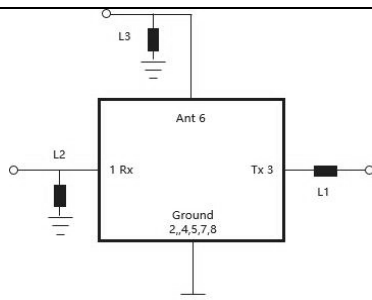
Figure 1 Electrical Characteristics: Tx to Ant.
